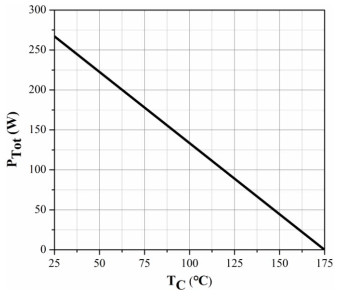
Figure 6. Power Derating
